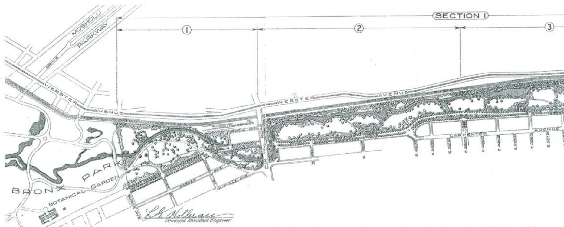
Bronx River Parkway Reservation, The Bronx to Kensico Dam, White Plains, Westchester County, NY. HAER NY-327, 18/22. Library of Congress
