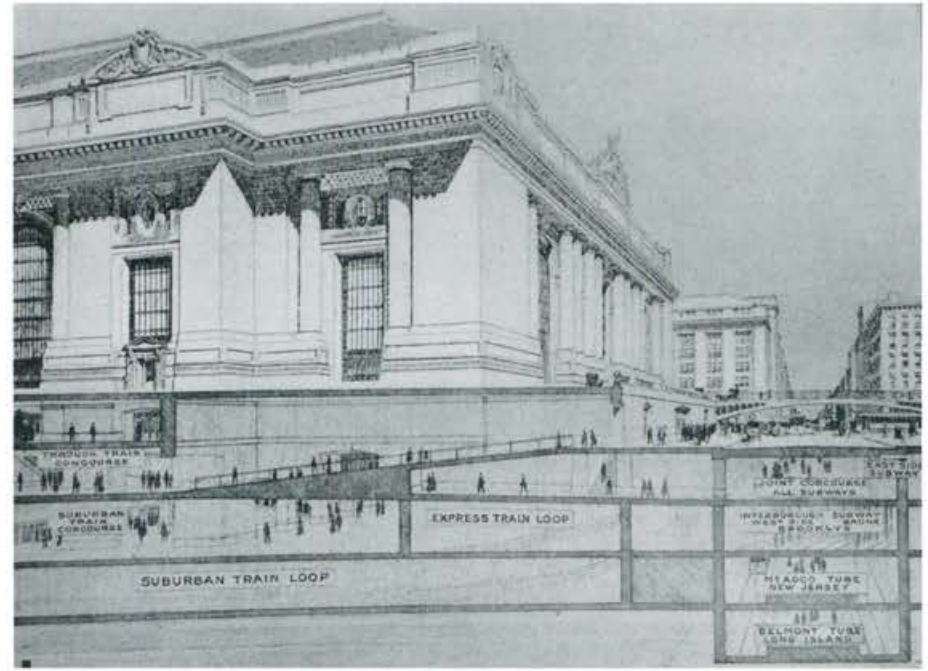
General sectional views of the Grand Central Terminal (1903-1913)
