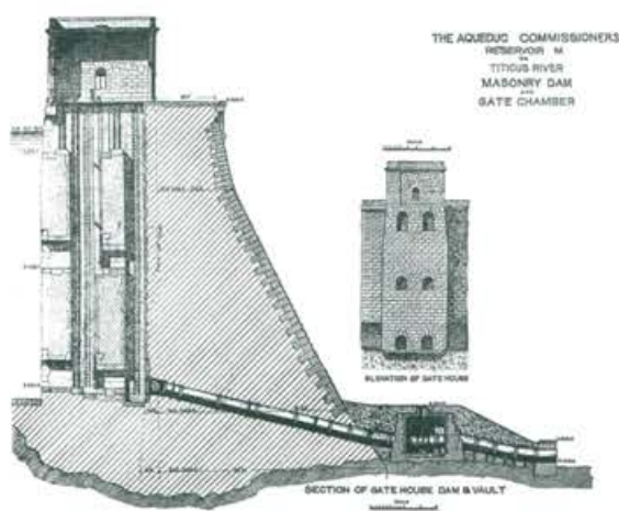
Titicus Dam
