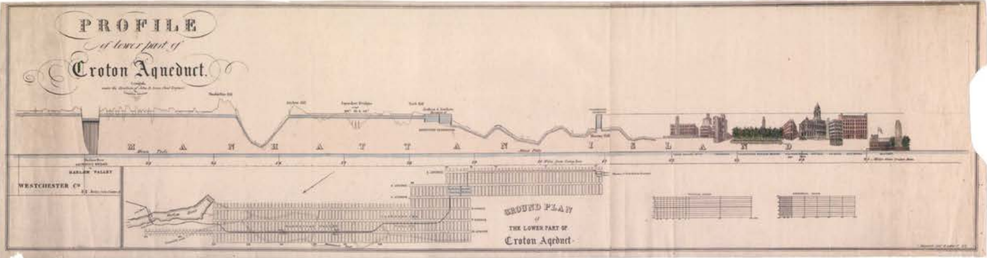
Profile and Ground Plan of the Lower Part of the Croton Aqueduct. by John Jervis
