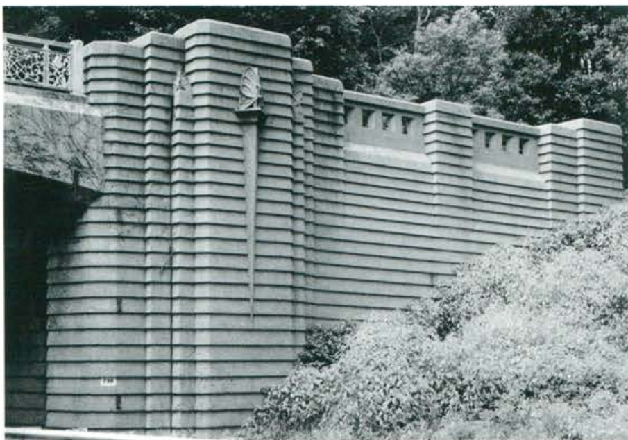
Detail of decorative abutment showing concrete butterflies. Merritt Parkway, Merwins Lane Bridge, Fairfield, Fairfield County, CT. HAER CONN,1-FAIRF,24-4. Library of Congress, Prints & Photographs Division
