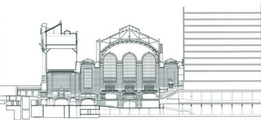
Grand Central Terminal Building Sections. Grand Central Terminal Design Guidelines © Metropolitan Transportation Authority
