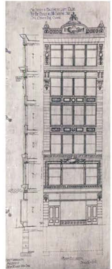
Front Elevation, 78 Greene Street, 1901.
