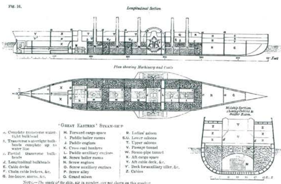
Longitudinal Section, Plan, and Midship Section of the 'Great Eastern' Steamship
