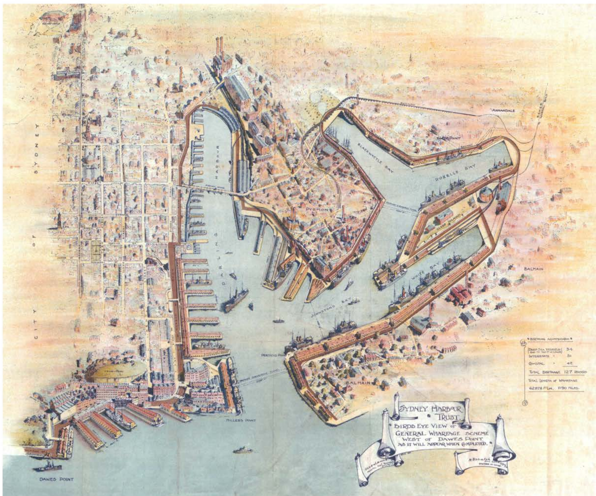
Lithograph, Bird's eye view of general wharfage scheme west of Dawes Point as it will appear when completed / Sydney Harbour Trust ; H.D. Walsh Engineer-in-chief 30/12/12 ; W. Adams, Principal asst. engineer 30/12/12 ; W.H.W. 1912. Sydney: McCarron, Stewart & Co., Printers and lithographers, 22-24-26 Goulburn St., 1912. Courtesy of National Library of Australia, nla.obj-232418156
