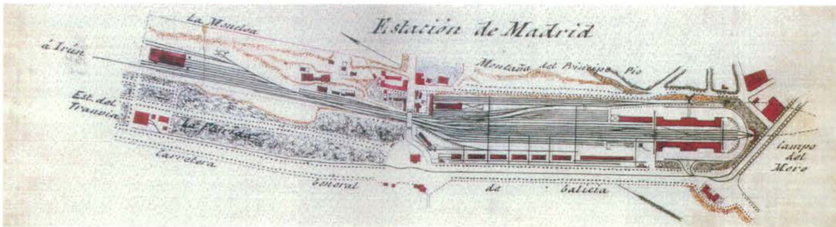
Layout of Principe Pio station, project of 1877 (prior to the definitive 1879), C.G.E.
