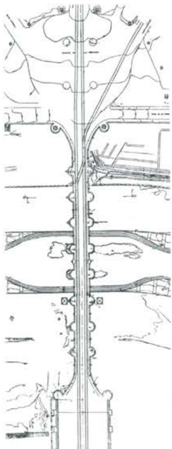
Toledo Bridge, according to Fernández Casado [92:607]
