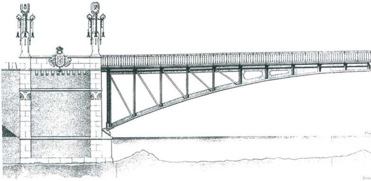
Princesa de Asturias Bridge in Madrid Machimbarrena and Beamonte
