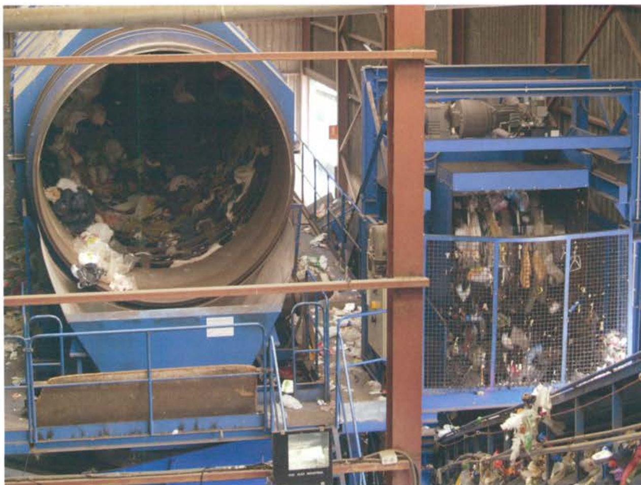
Rotary screen for volumetric separation at the Pinto Packaging Sorting Plant.
