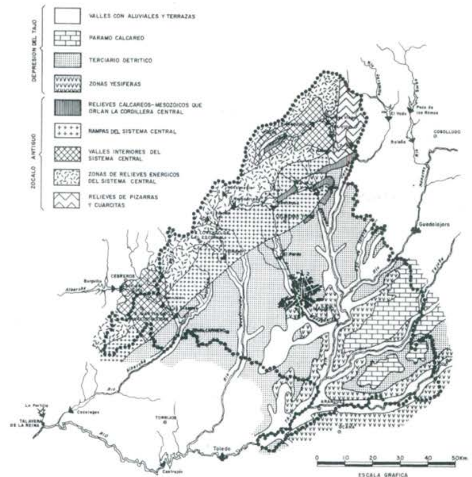
Geomorphology of Madrid
