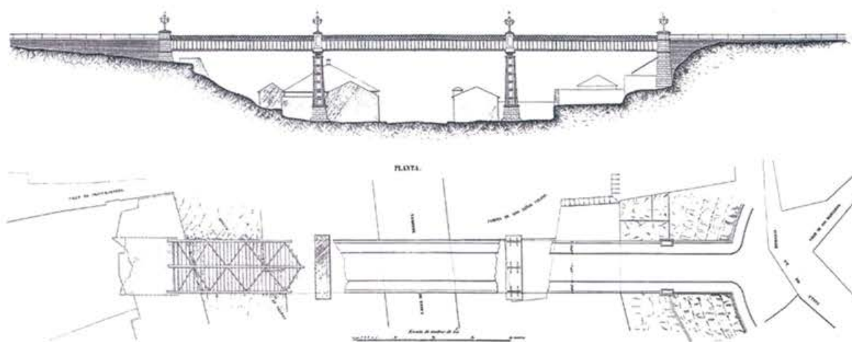
Iron viaduct on the Calle Bailén in Madrid (Barrón, 1872) [ROP 1861,271]
