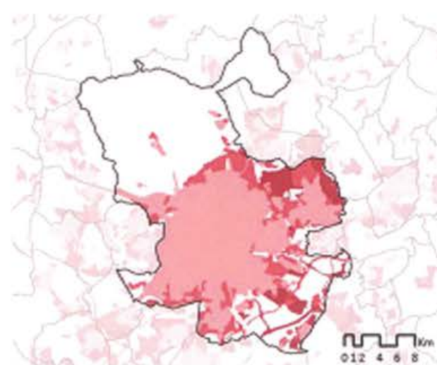
Artificial surface evolution. 1987-2010 Corine Land Cover. (light pink 1987, darker pink 2000 and wine-red 2006)
