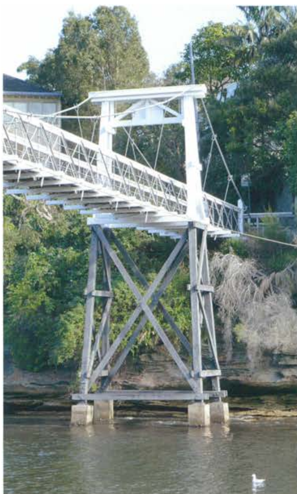
Parsley Bay Suspension Bridge, 1910
