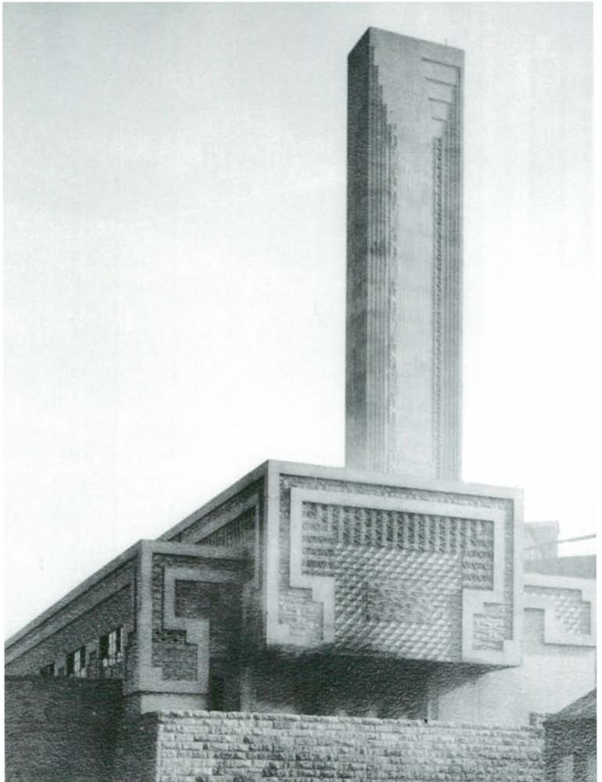
Exterior view of Pymont Incinerator from south-west, Sydney. Walter Burley Griffin & Eric M. Nicholls, 1935. Courtesy of National Library of Australia, nla.obj-150422021
