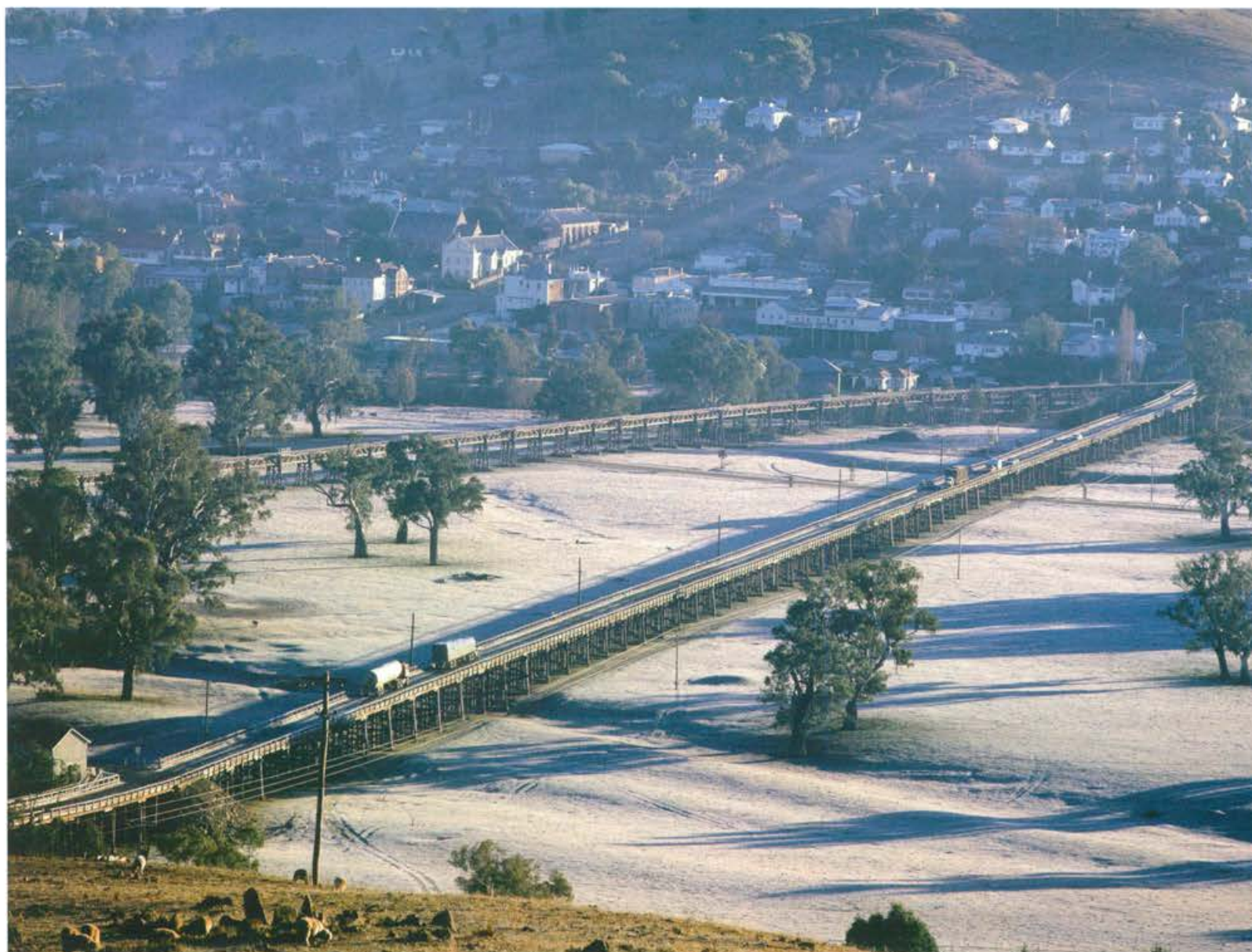
Hume Highway Duplication crossed the Murrumbidgee River flood plain at Gundagai by a long narrow timber trestle structure. RTA Transparency. Mike Pratt, 1976. Courtesy of Transport Roads & Maritime Services, NSW Government
