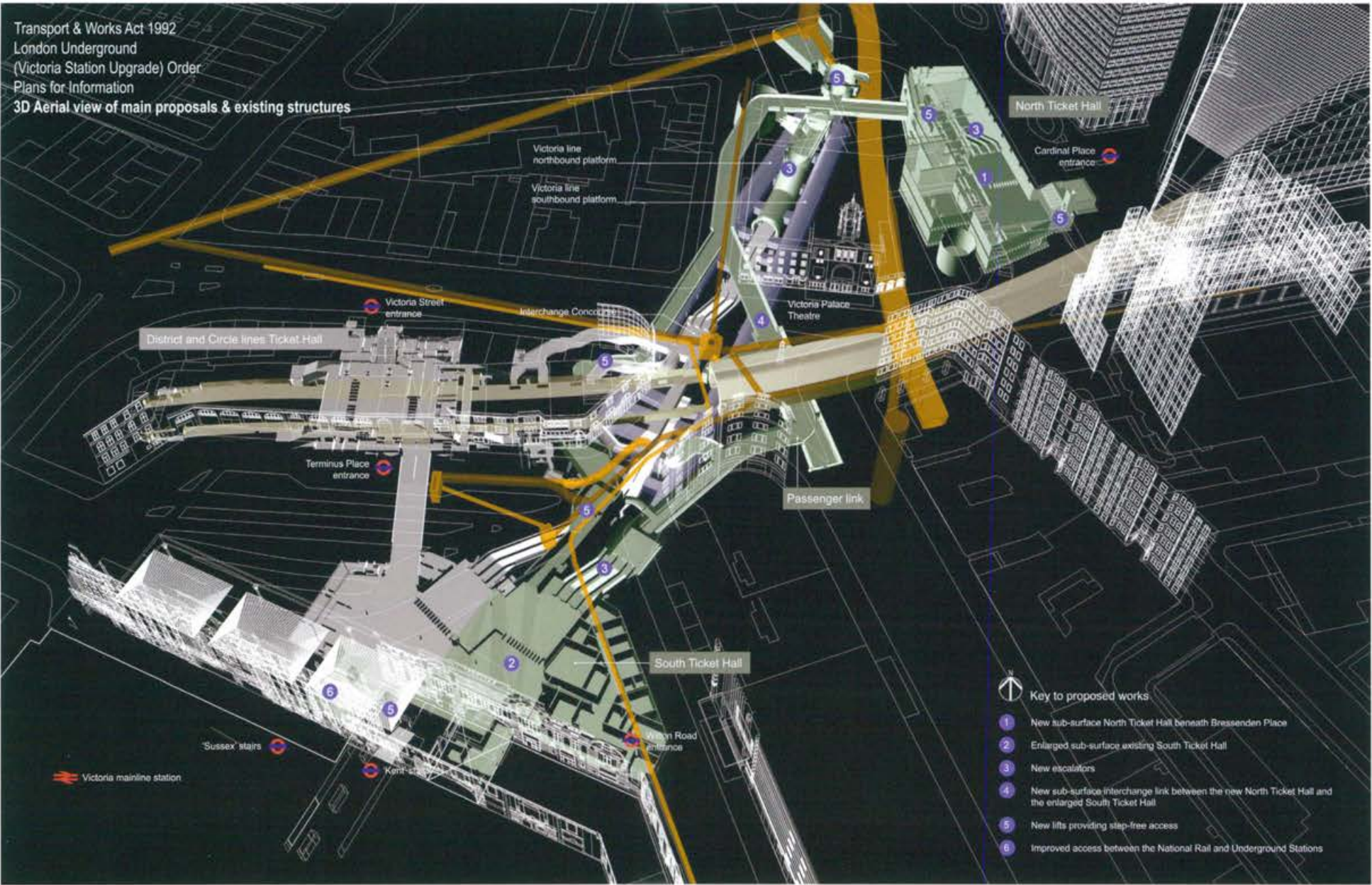
Esquema de Victoria Station [London Bridge Associates LTD, https://www.lba.london/project/victoria-station-upgrade/ ]
