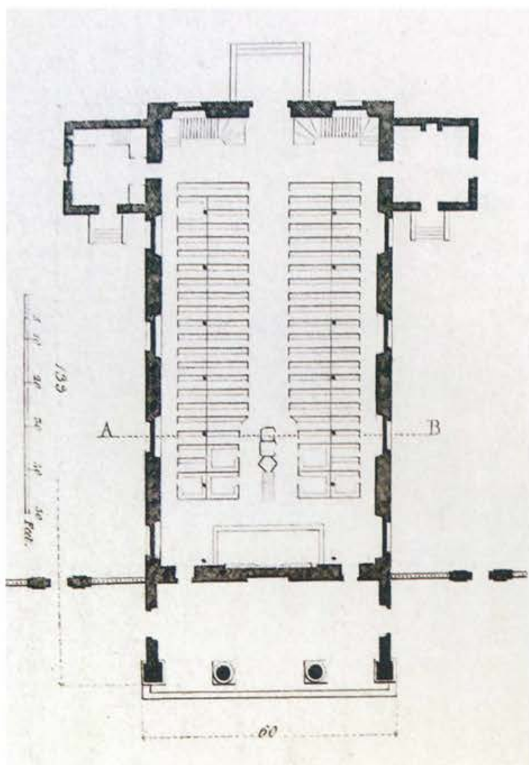
St Paul's Church, Covent Garden – planta y alzado este [105:115, vol.I]
