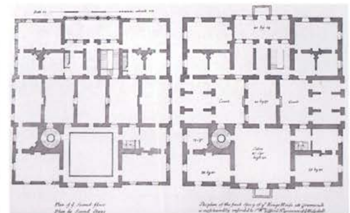
Queen's House - planta
