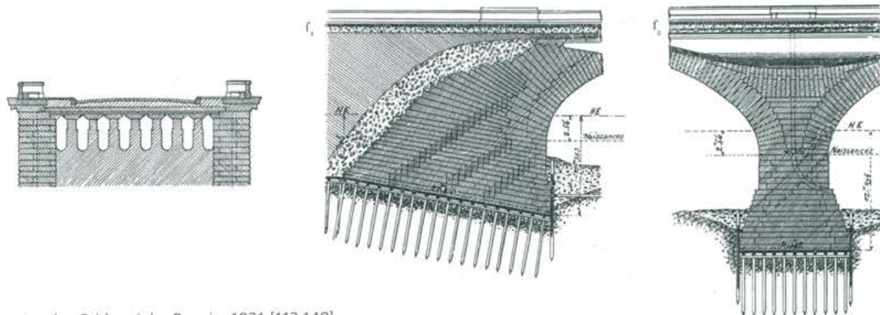
London Bridge, John Rennie, 1831 [113:148]
