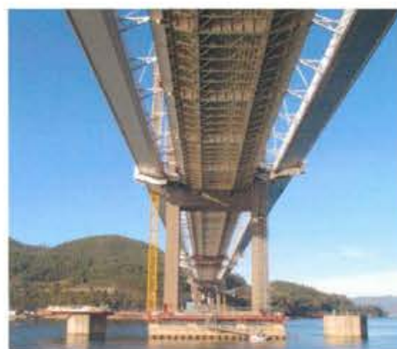
AP-9 highway link Cangas-Teis, Galicia. 2017
