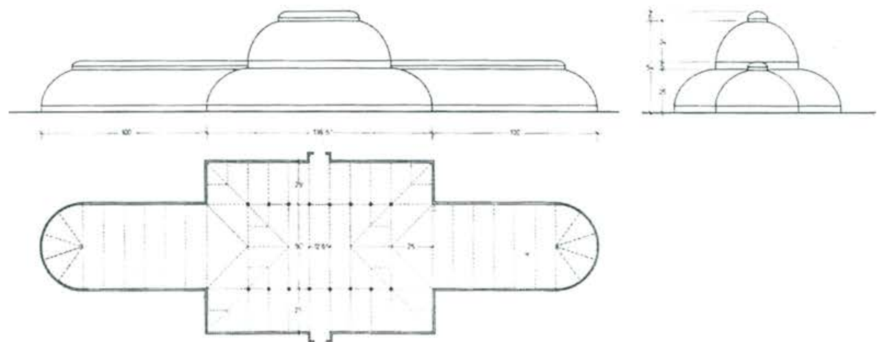
Plan and section, Palm House, Kew Gardens (Richard Turner, 1844) 29
