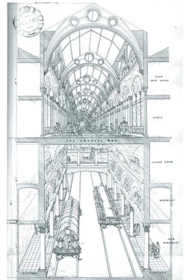
The Crystal Way, Moseley, 1855 [Report from the Select Committee on Metropolitan Communications. London, House of Commons 1855]
