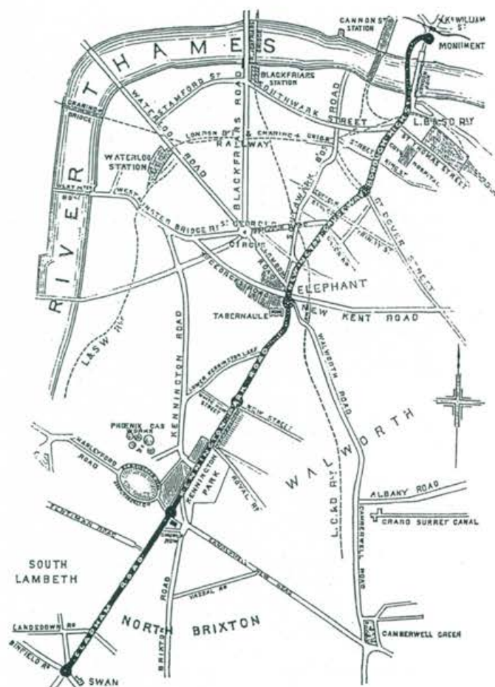
City & South London Railway-Barrier and cut of the accesses to London from Southwark
