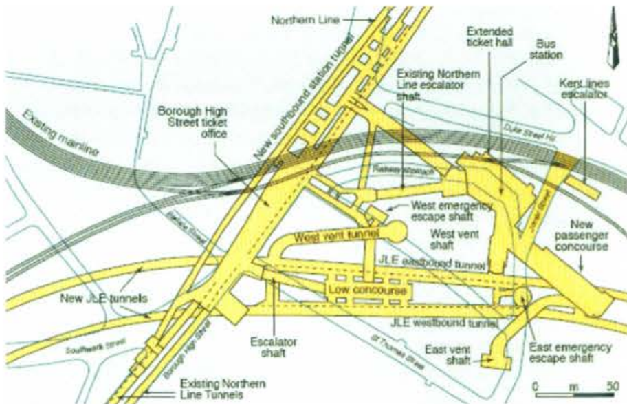
Waterloo and London Bridge [112:122]
