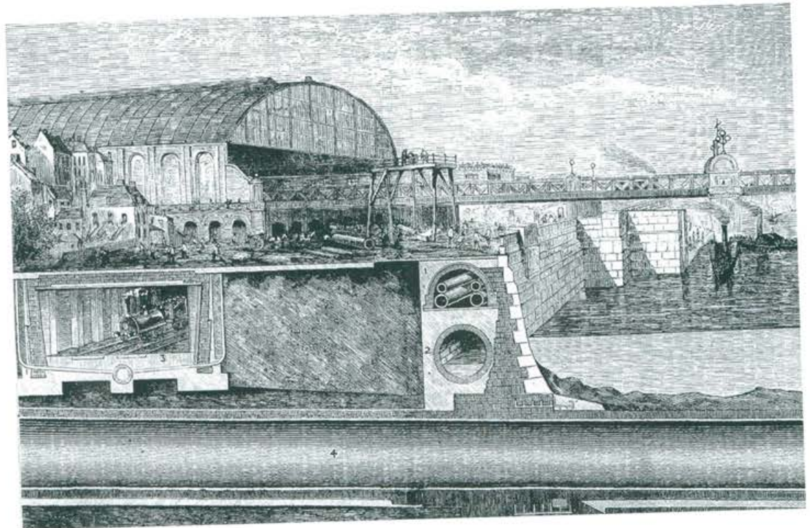
Victoria Embankment, section, 1867[61:159]
