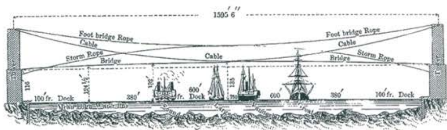
Front view of the bridge showing the temporary ropes employed for the system of cables
