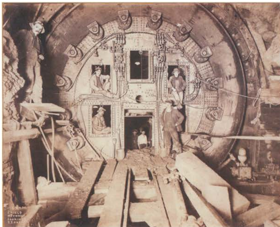
Transportation Hudson tubes [Boring shields by which Hudson River tunnels were excavated.] 1908.
