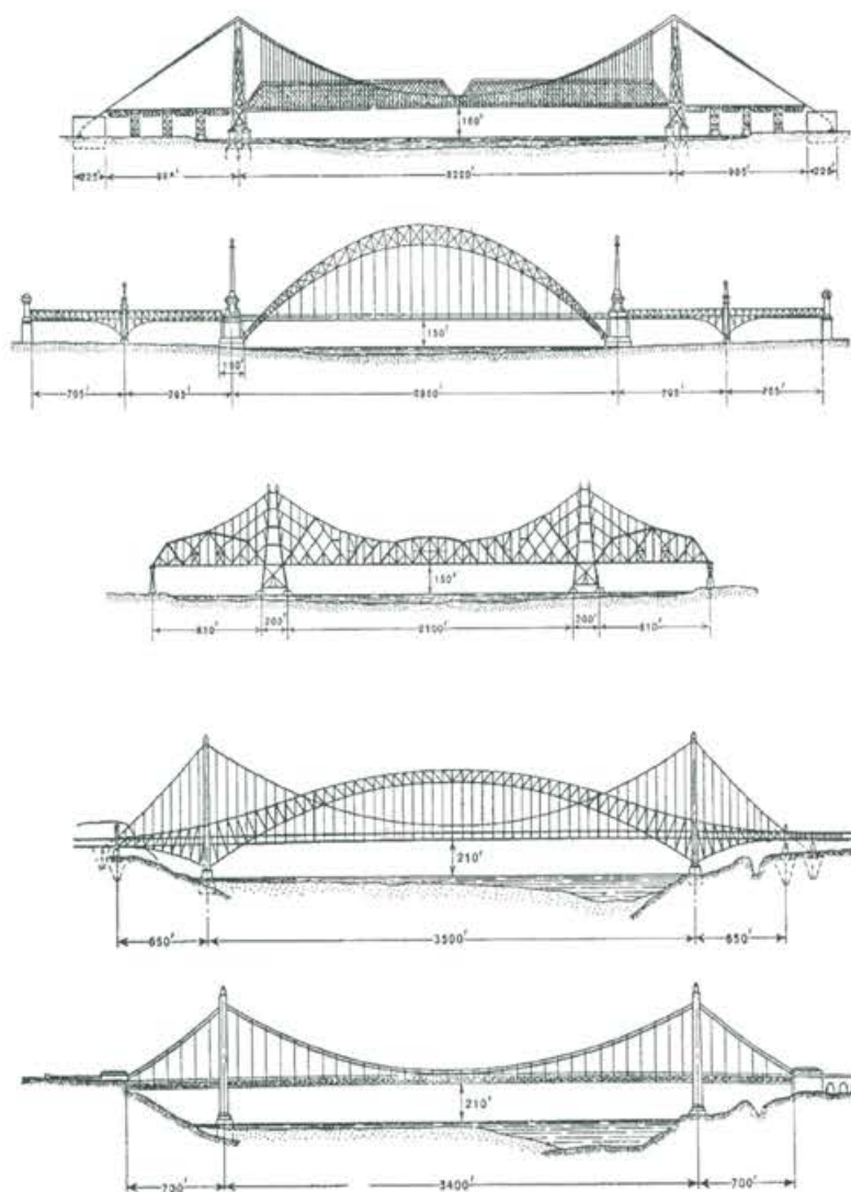
Proposed bridge over the Hudson, Gustav Lindenthal [110: 92-95]
