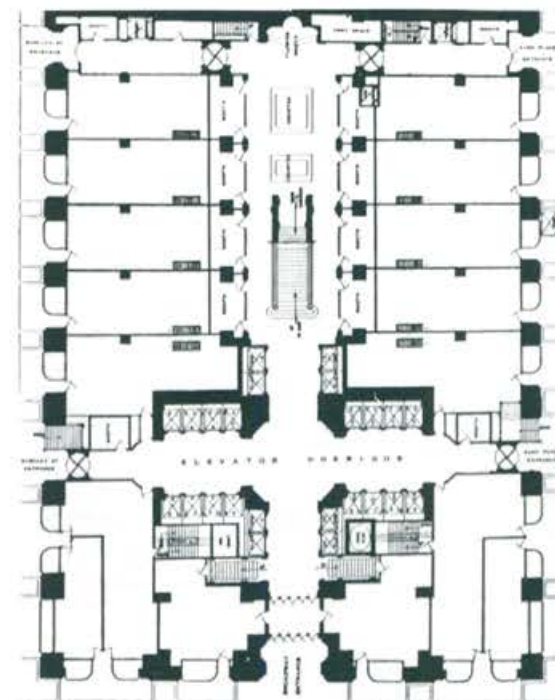
Woolworth Building: Plan ground floor, by Cass Gilbert.
