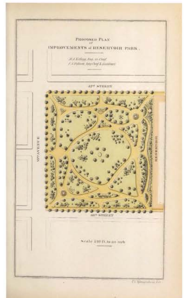
Spangenberg, Charles. Proposed plan of improvements of Reservoir Park, 1871.
