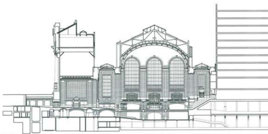
Grand Central Terminal Building Sections. Grand Central Terminal Design Guidelines © Metropolitan Transportation Authority. Used with permission.
