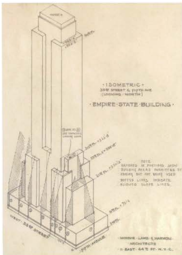
Empire State Building. Isometric 33rd street and 5th Ave. (looking North). Harold Rider Collection, ArchiTech Gallery.
