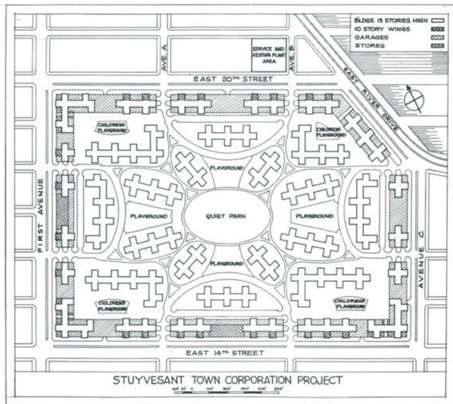
Plan, Stuyvesant Town Corporation Project: E. 14th Street to E. 20th Street; 1st Avenue to Avenue C; East River Drive. Courtesy NYC Municipal Archives.
