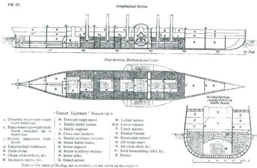
Longitudinal Section, Plan, and Midship Section of the 'Great Eastern' Steamship Marine & Aviation, Pier 57
