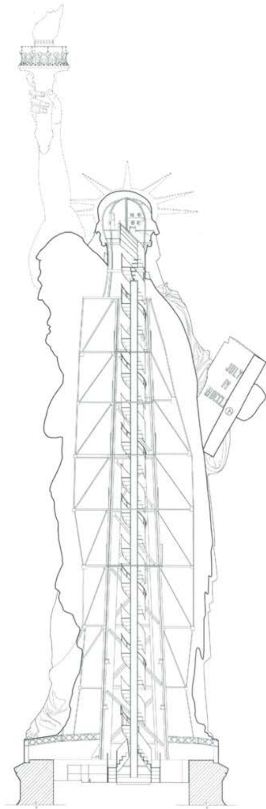
Statue of Liberty (Bartholdi & Eiffel, 1886). Sculptor Frédéric Auguste Bartholdi (1834-1904) and engineer Gustave Eiffel (1832-1923), according to Condit, it is the first use of steel in the United States after the Brooklyn Bridge [33:117]
